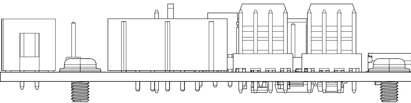
View from Left side (Scale 5:2)
