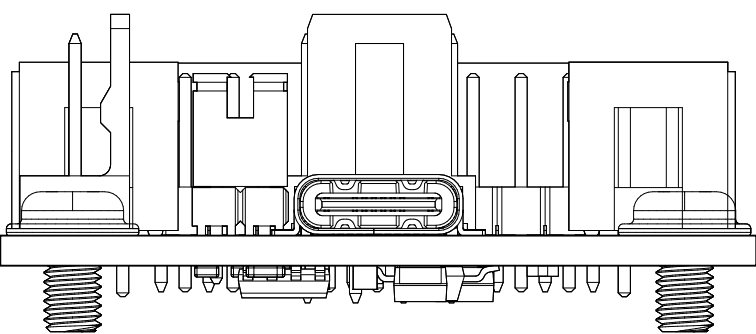
View from Front side (Scale 5:2)
